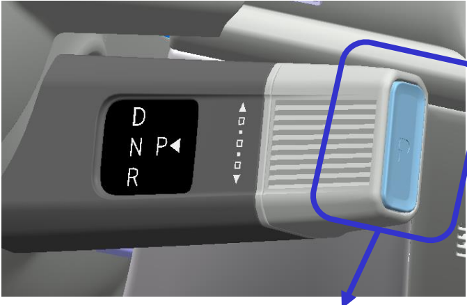
“P” parking position button
